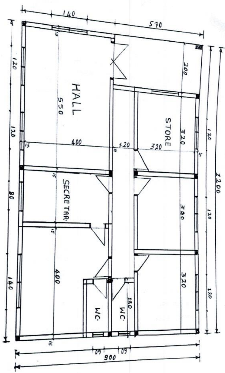
GROUND PLAN
